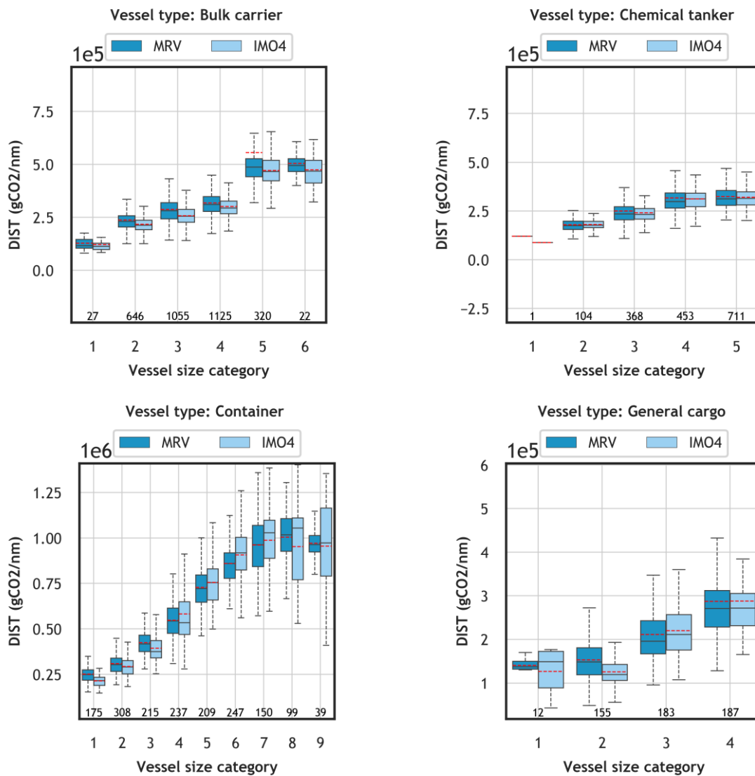
Figure 73 - Box plot distance carbon intensity comparison by vessel type and size
