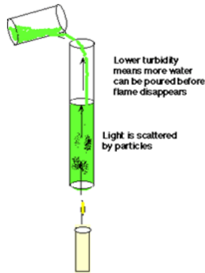
Figure 10. A Jackson Candle Turbidimeter
