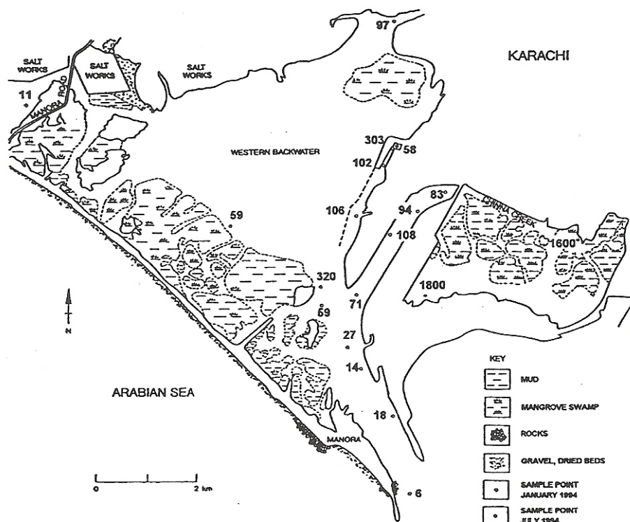
Figure 2; Distribution of copper in Karachi Harbour sediments
