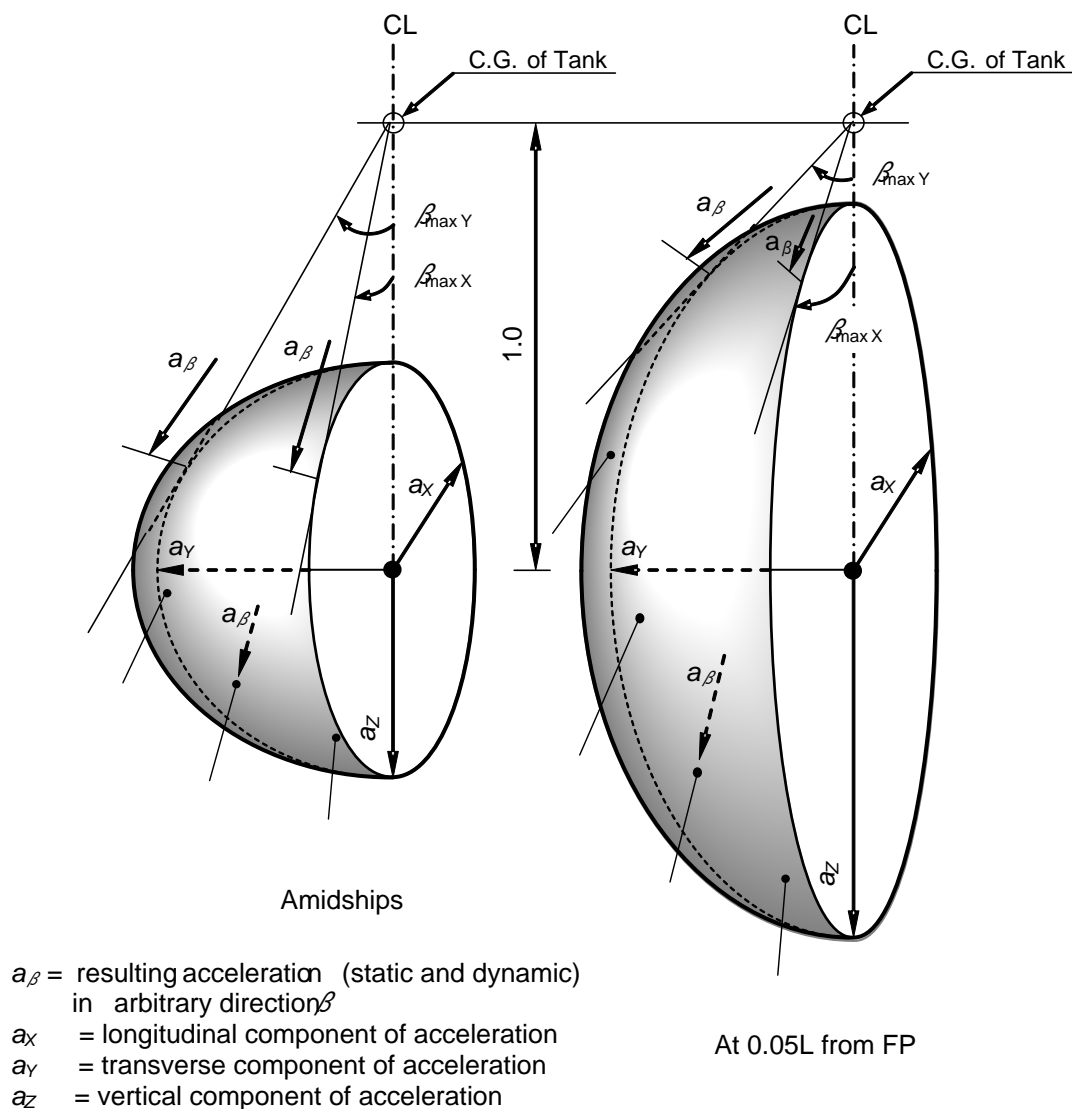
Figure 4.1 – Acceleration ellipsoid
