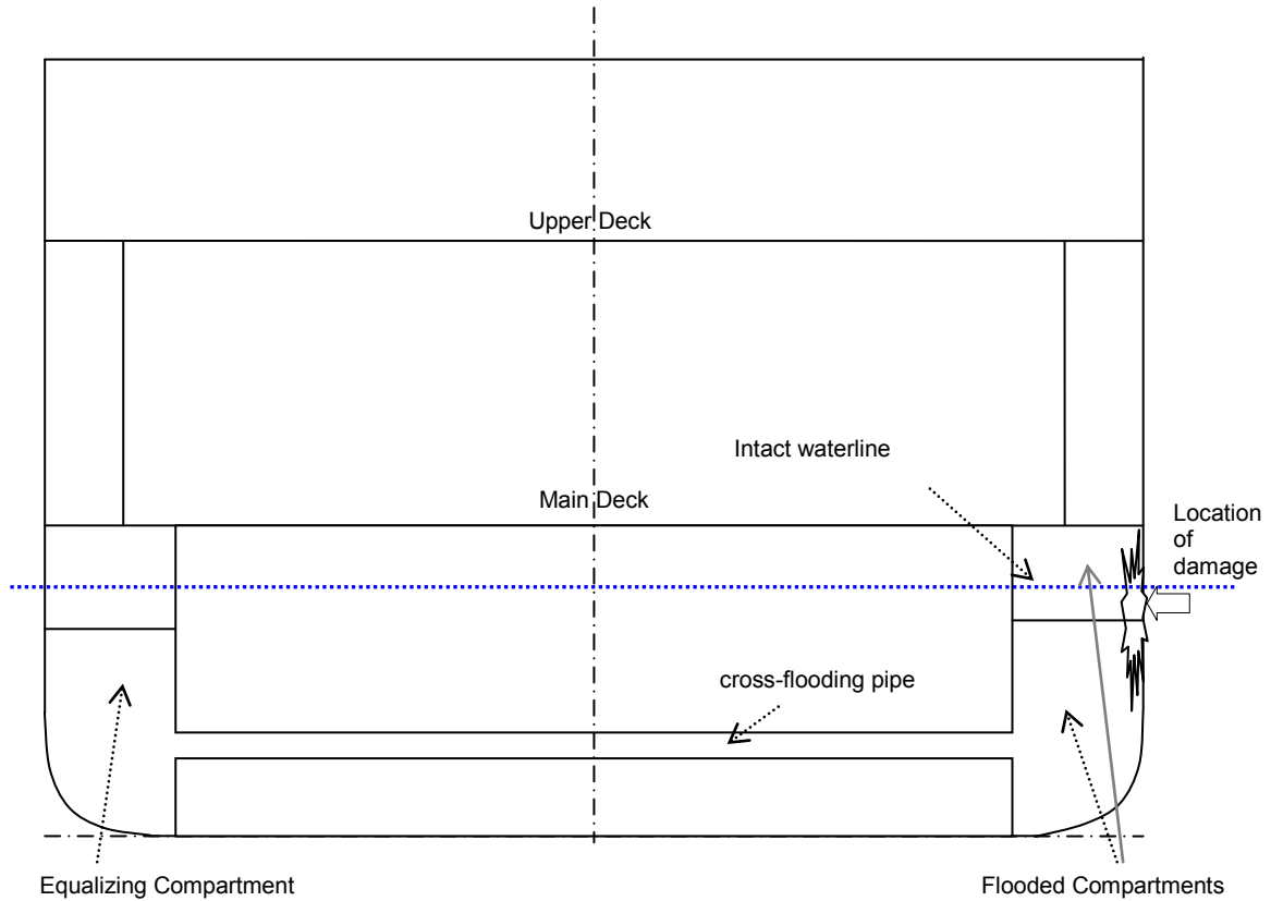
Figure 1(a) – Section showing cross-flooding pipe and compartments
