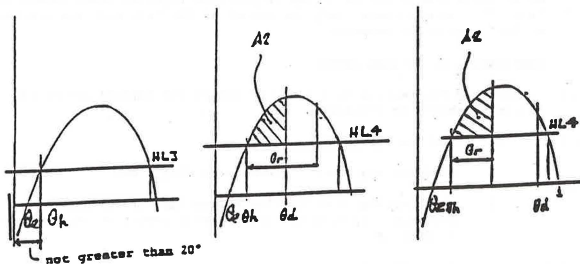
Figure 2 - Damage stability
