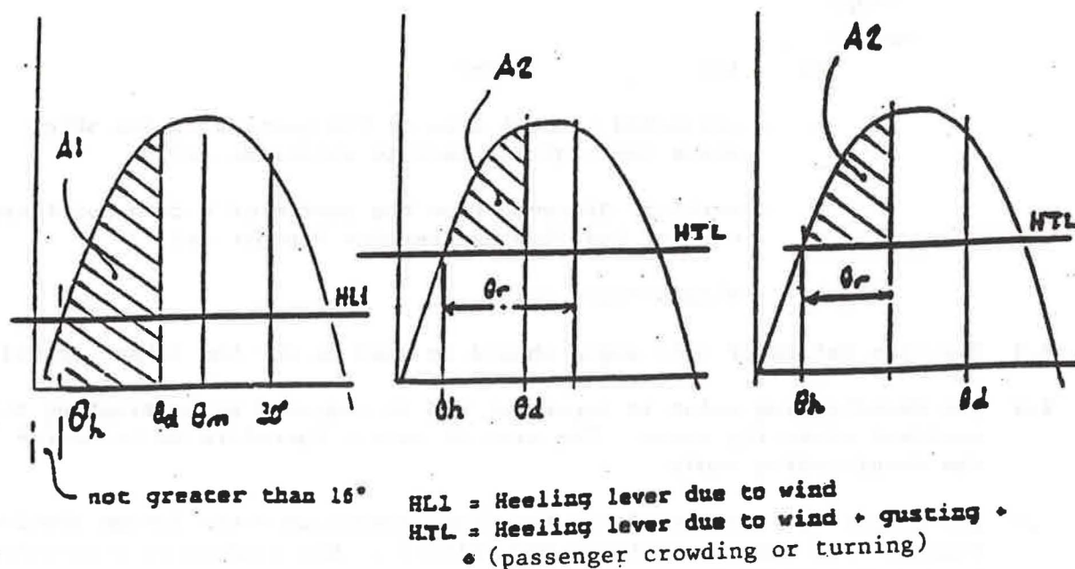
Figure 1 - Intact stability
