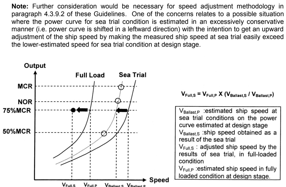
Figure 2: An Example of Possible Ship Speed Adjustment
