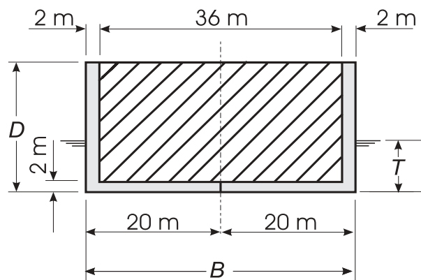
Midship section
