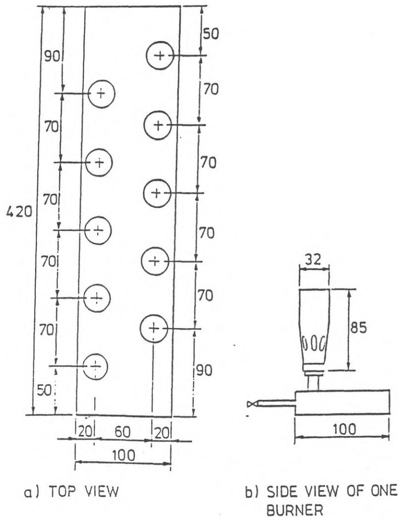
FIG. 1 FIRE ENDURANCE TEST BURNER ASSEMBLY
