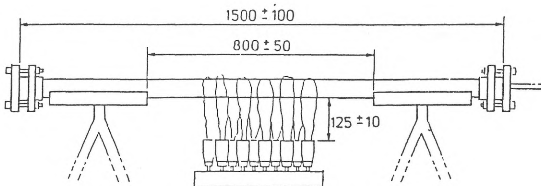
FIG. 2 FIRE ENDURANCE TEST. STAND WITH MOUNTED SAMPLE
