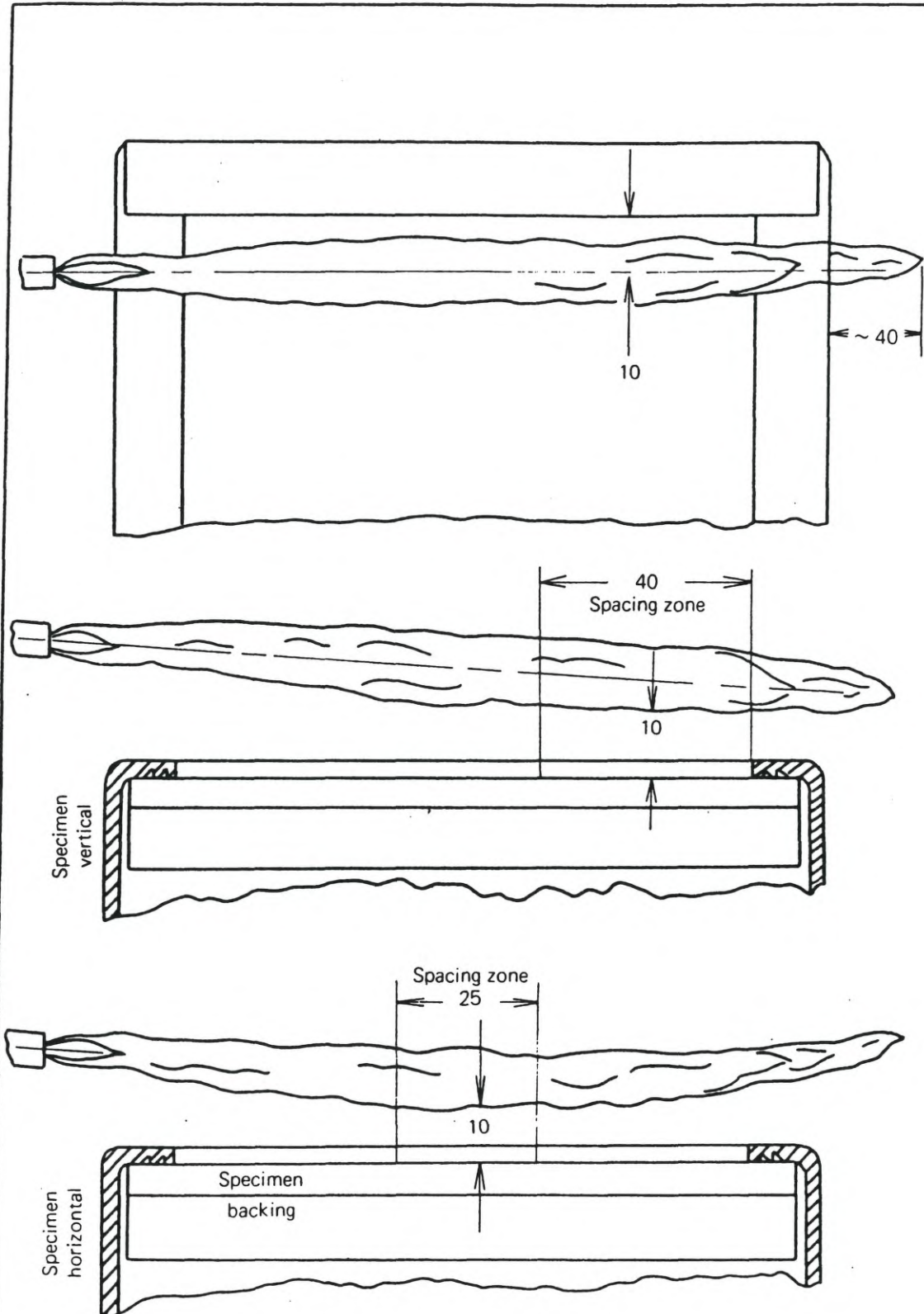
Figure 9 — Position of pilot flame
